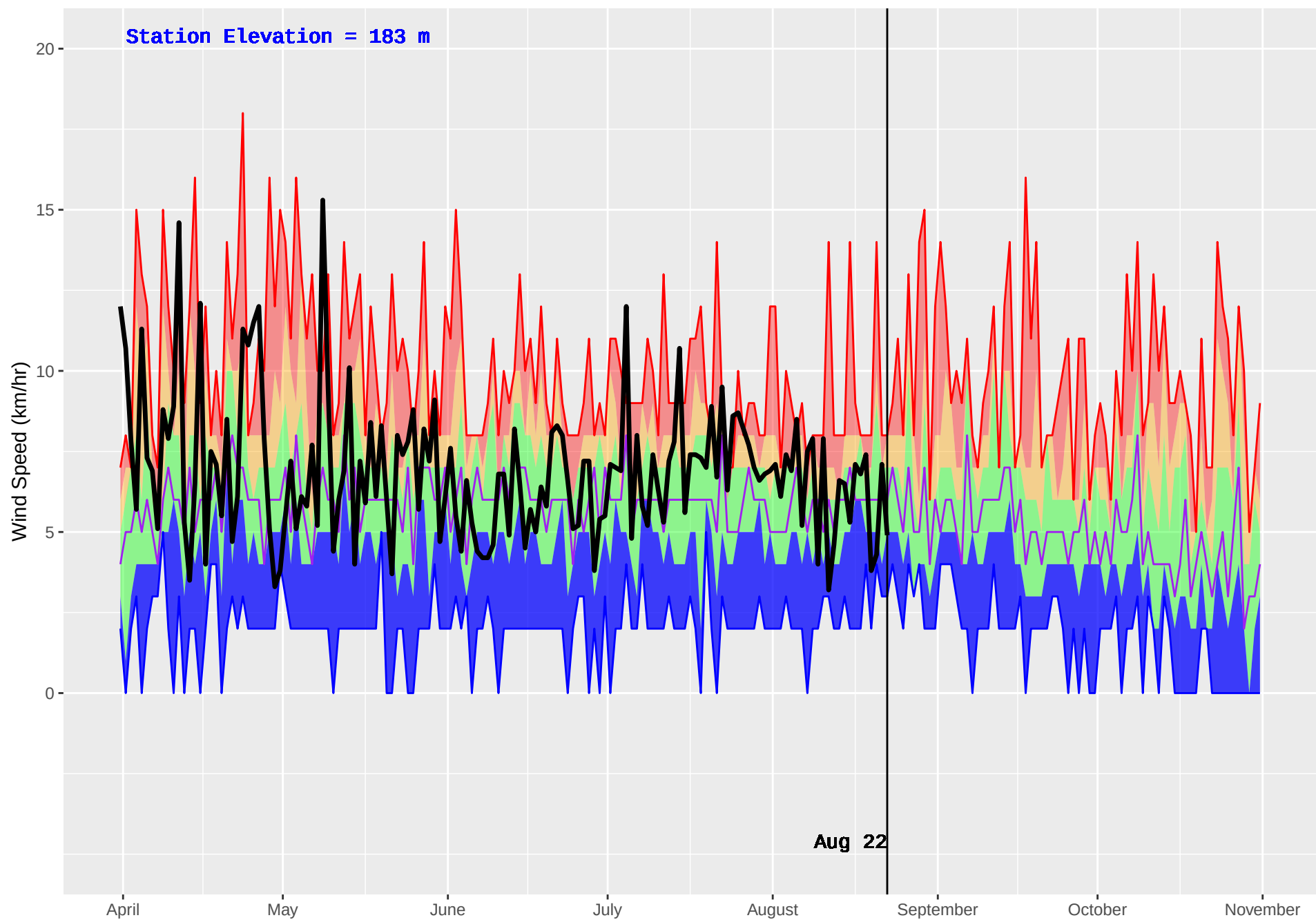
MESACHIE 2 (934) : Historical (2006–2016) and Current (2018) Daily Wind Speed
